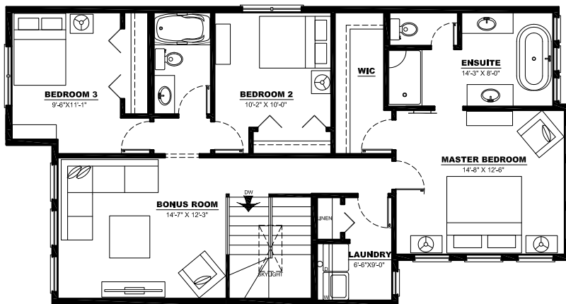
UPPER FLOOR PLAN = 1150 SQ FT
