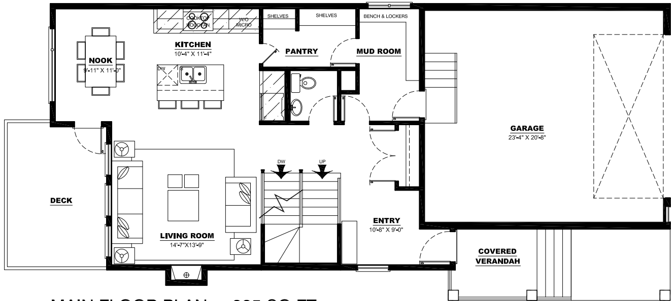
MAIN FLOOR PLAN = 885 SQ FT
