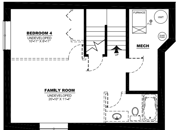
LOWER FLOOR PLAN = 560 SQ FT
