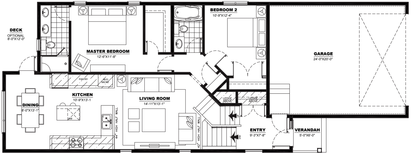
MAIN FLOOR PLAN: 1150 SQ FT
