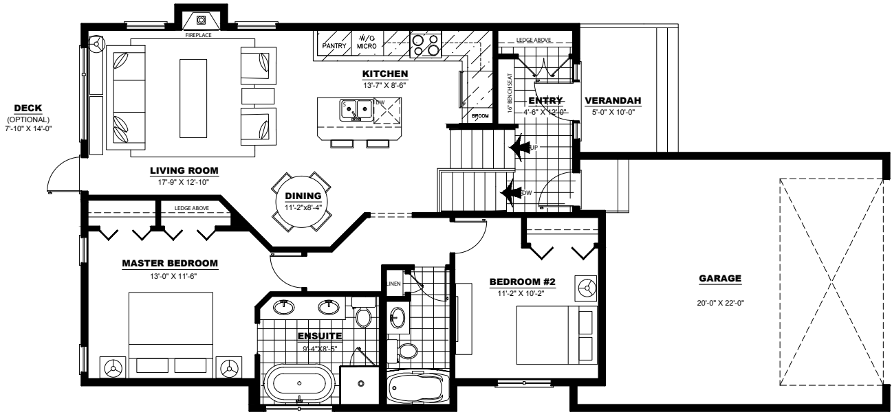
MAIN FLOOR PLAN: 1137 SQ. FT.
