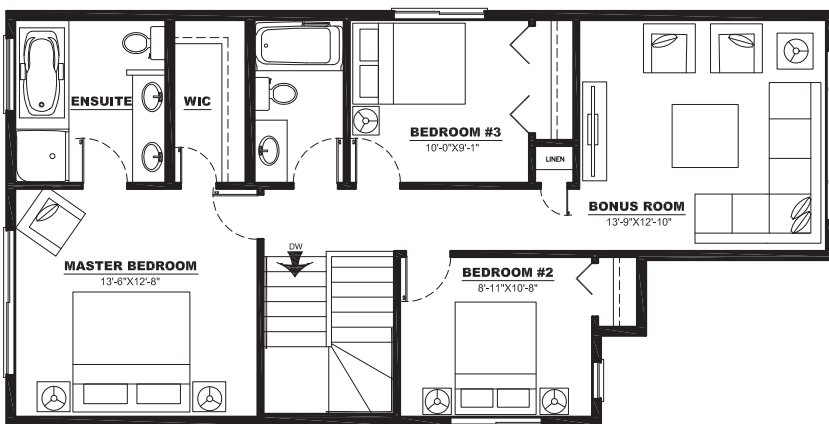
UPPER FLOOR PLAN: 949 SQ. FT.
