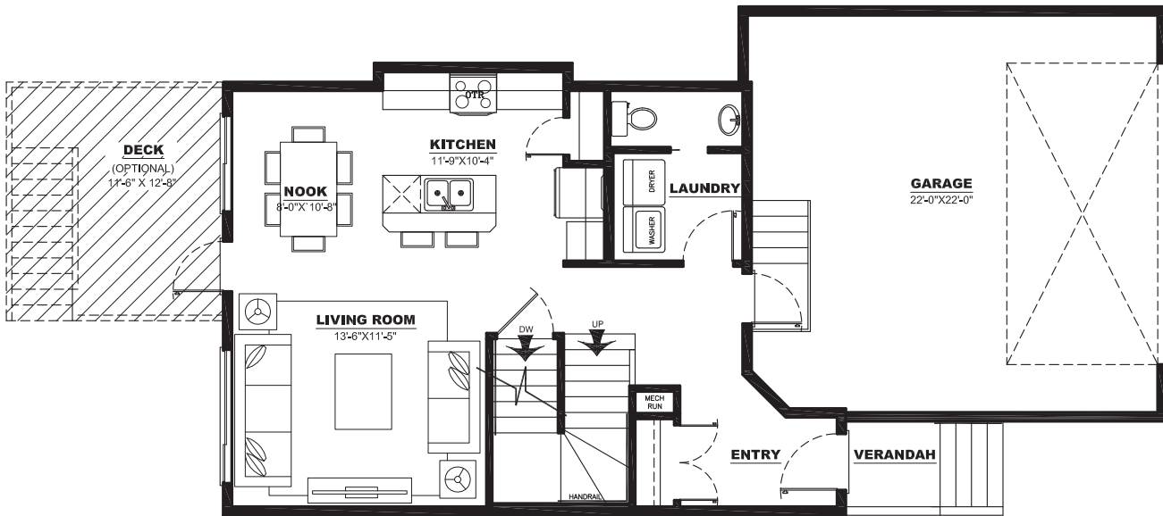
MAIN FLOOR PLAN: 685 SQ. FT.
