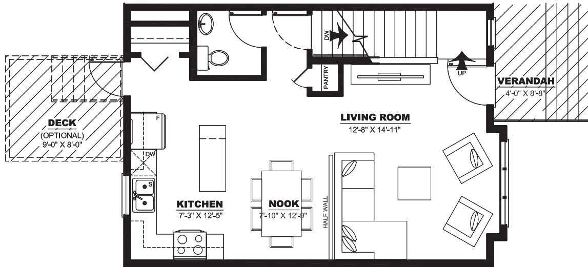
MAIN FLOOR PLAN: 569 SQ. FT.
