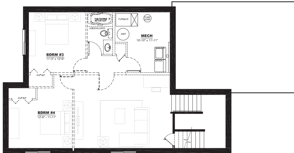
LOWER FLOOR PLAN: 770 SQ. FT.
