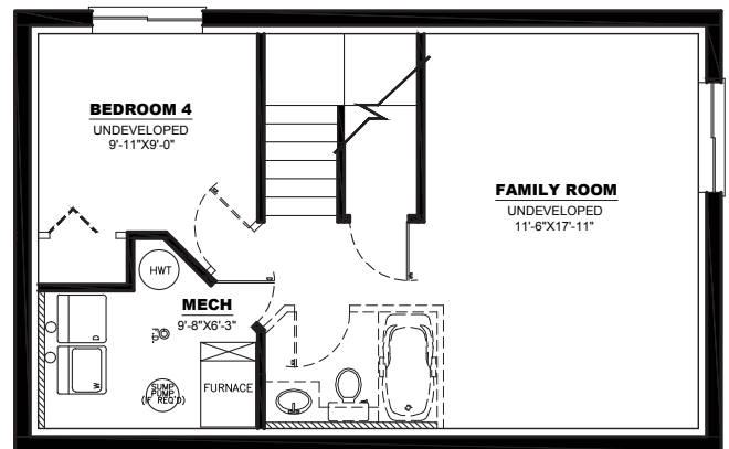
LOWER FLOOR PLAN: 484 SQ FT
