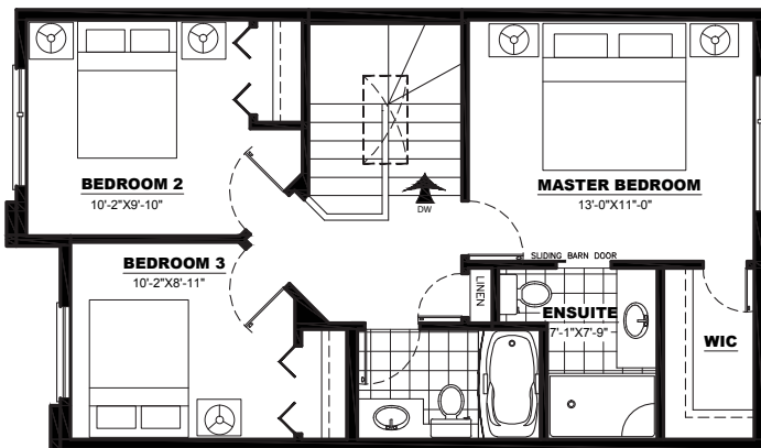
UPPER FLOOR PLAN: 662 SQ FT
