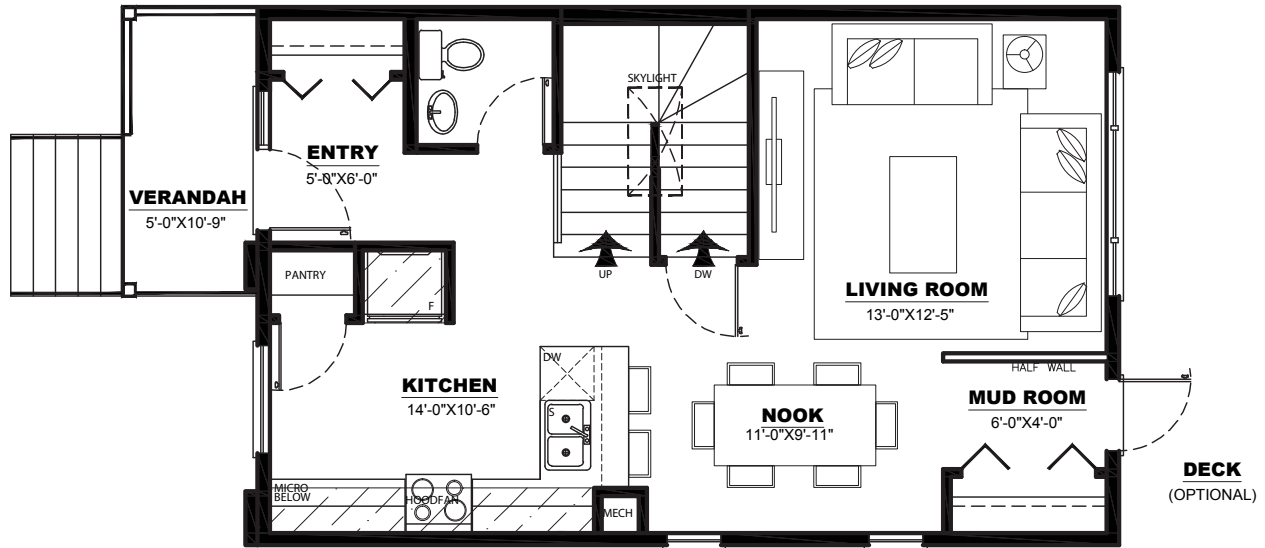
MAIN FLOOR PLAN: 640 SQ FT
