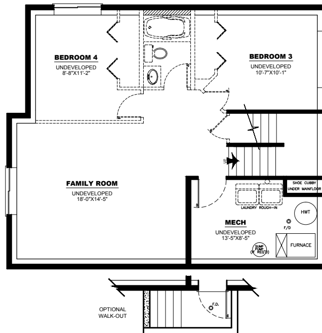
LOWER FLOOR PLAN: 708 SQ FT
