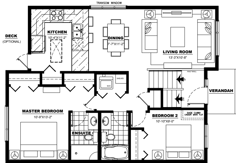
MAIN FLOOR PLAN: 985 SQ FT
