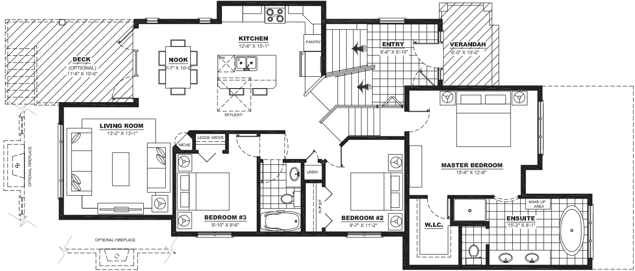
MAIN FLOOR PLAN: 1424 SQ FT
