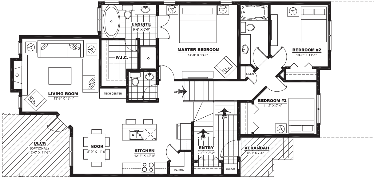
MAIN FLOOR PLAN: 1398 SQ FT
