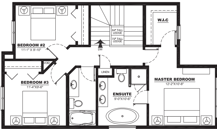
UPPER FLOOR PLAN: 475 SQ FT
