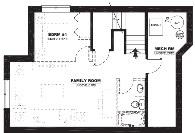
LOWER FLOOR PLAN: 811 SQ FT
