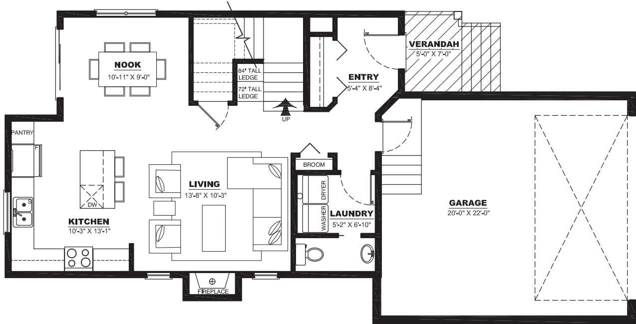
MAIN FLOOR PLAN: 723 SQ FT
