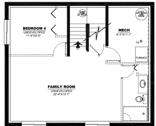
LOWER FLOOR PLAN: 558 SQ FT
