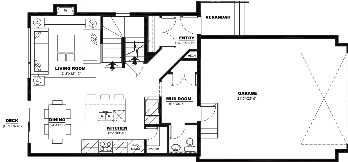
MAIN FLOOR PLAN: 757 SQ FT
