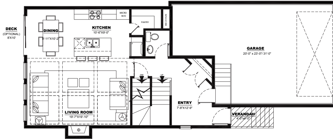
MAIN FLOOR PLAN: 767 SQ FT
