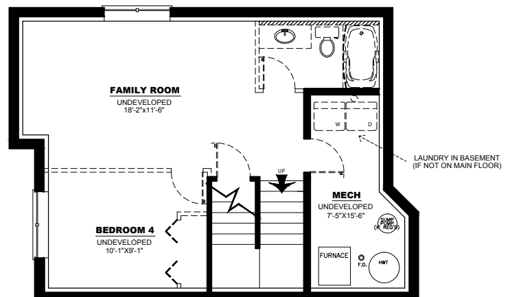
LOWER FLOOR PLAN: 480 SQ FT
