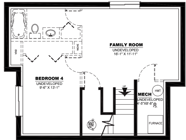
LOWER FLOOR PLAN: 500 SQ FT
