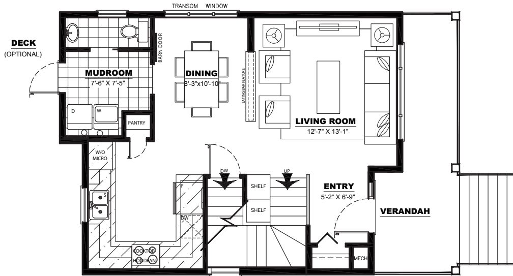
MAIN FLOOR PLAN: 644 SQ FT
