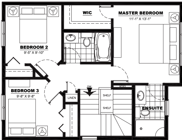
UPPER FLOOR PLAN: 667 SQ FT
