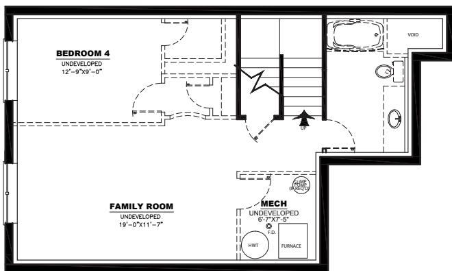
LOWER FLOOR PLAN: 595 SQ FT
